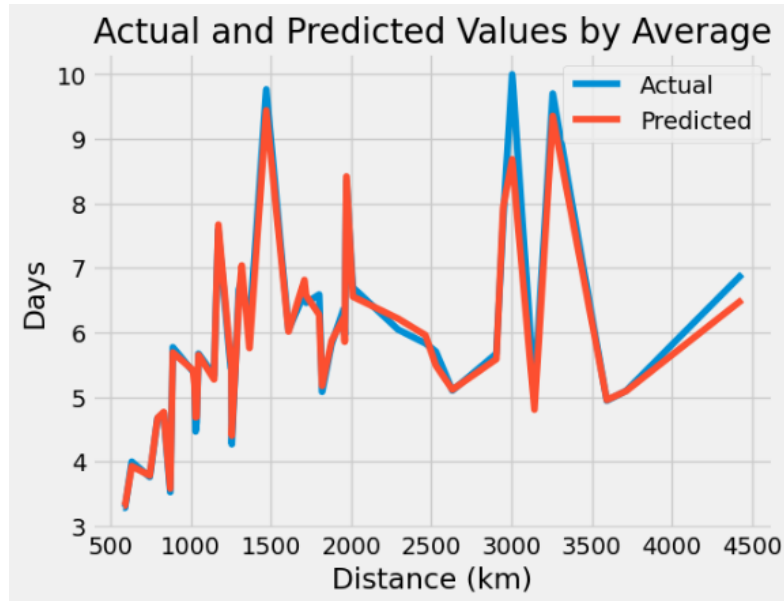
Figure 6. Actual and Predicted Average Scores Scenario 1
