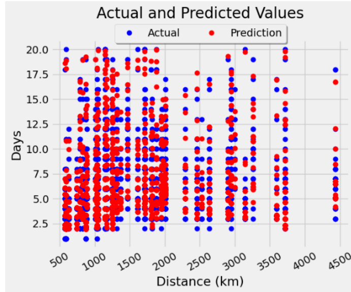
Figure 8. Plot Actual and Predicted Values FR Scenario 2
